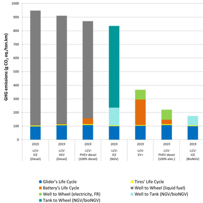
Figure 14: Potential impact on climate change for light commercial vehicles – 2019 time horizon
