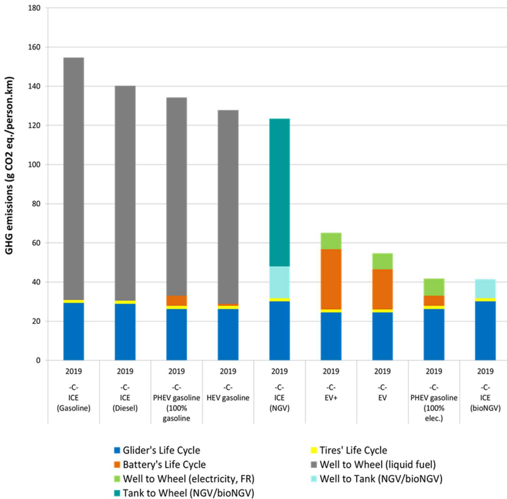
Figure 8: Potential impact on climate change for C-segment vehicles in 2019
