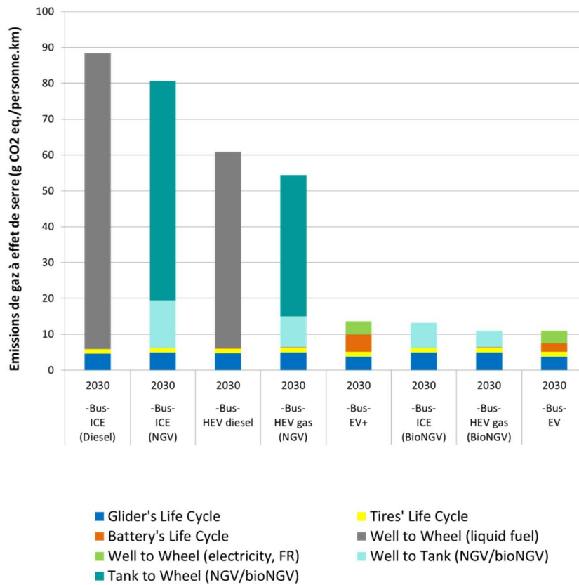
Figure 13: Potential impact on climate change for buses – 2030 time horizon
