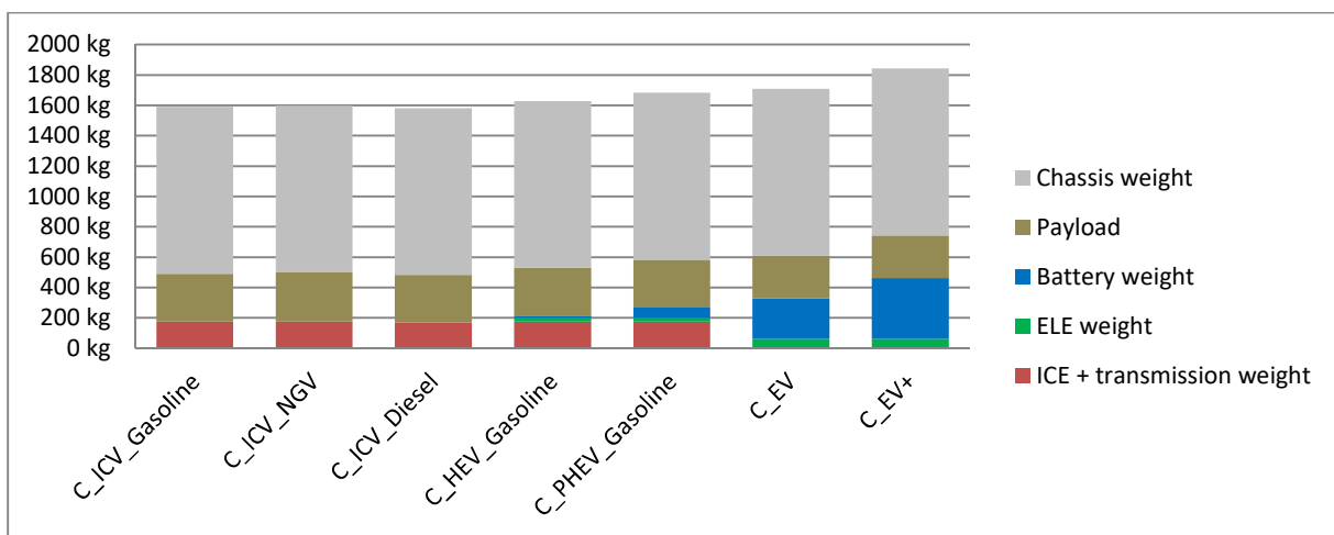
Figure 4: Weight breakdown of C segment vehicles 2019 (ELE: Electric engine - ICE: Internal combustion engine - the payload is determined by reference to the European WLTP test protocol plus the tank taken into account)
