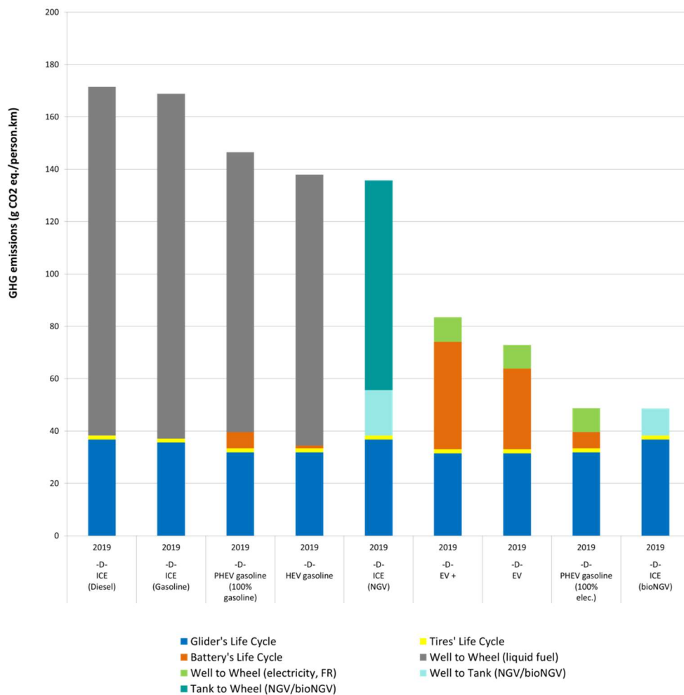
Figure 10: Potential impact on climate change for D-segment vehicles in 2019
