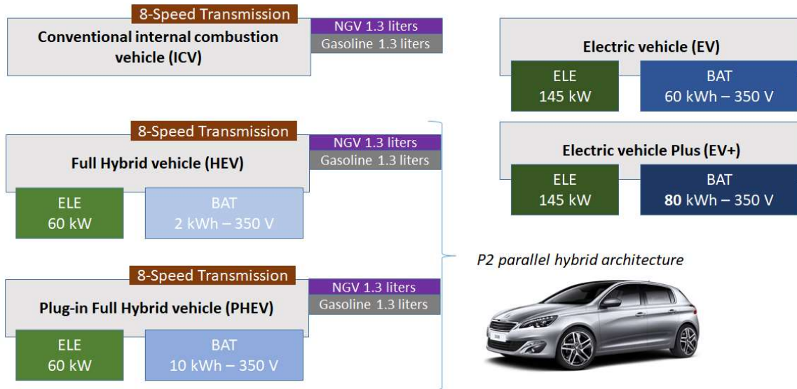
Figure 3: Design of C segment architecture (ELE: electric engine, BAT: Battery)
