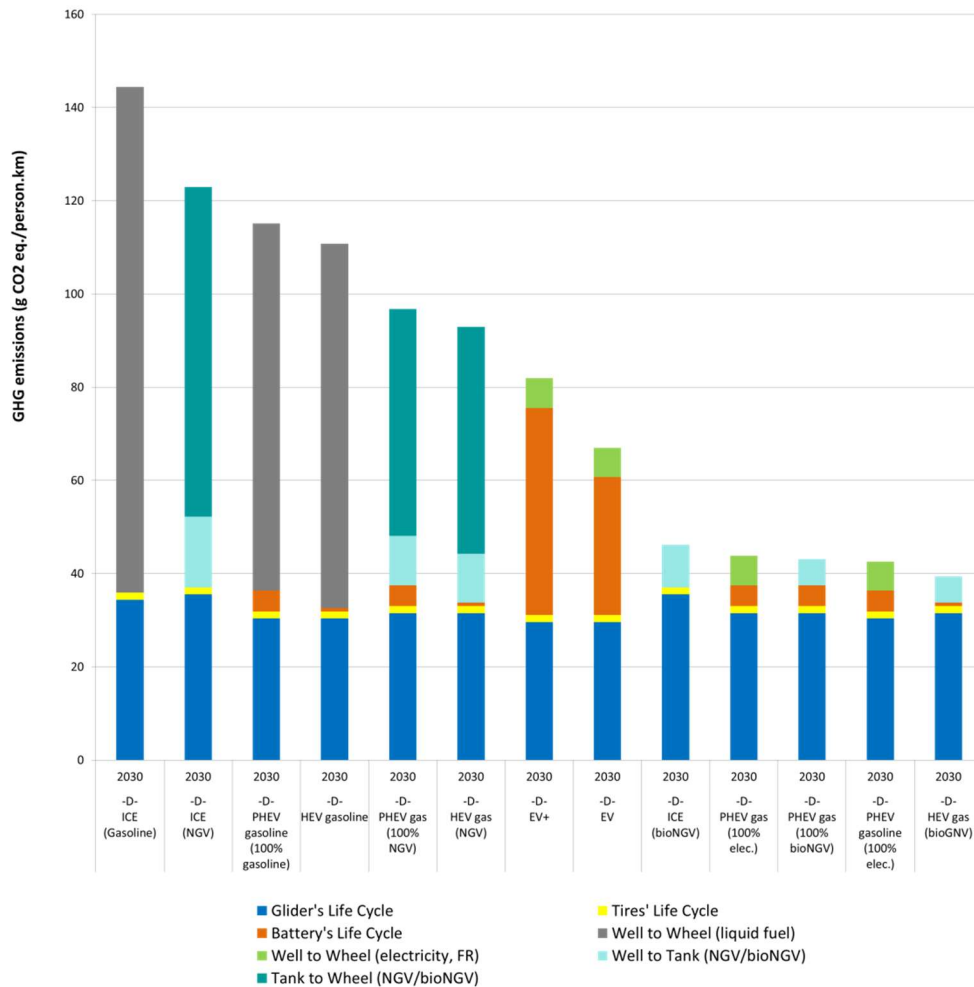
Figure 11: Potential impact on climate change for D-segment vehicles in 2030
