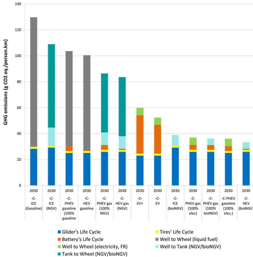
Figure 9: Potential impact on climate change for C-segment vehicles in 2030
