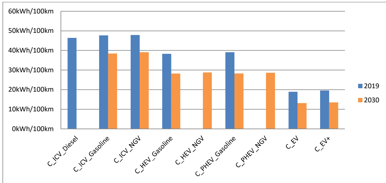
Figure 6: Energy consumption [kWh/100 km] of C segment vehicles – 2019
