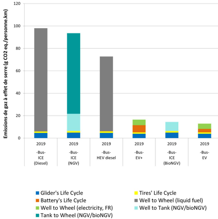
Figure 12: Potential impact on climate change for buses – 2019 time horizon
