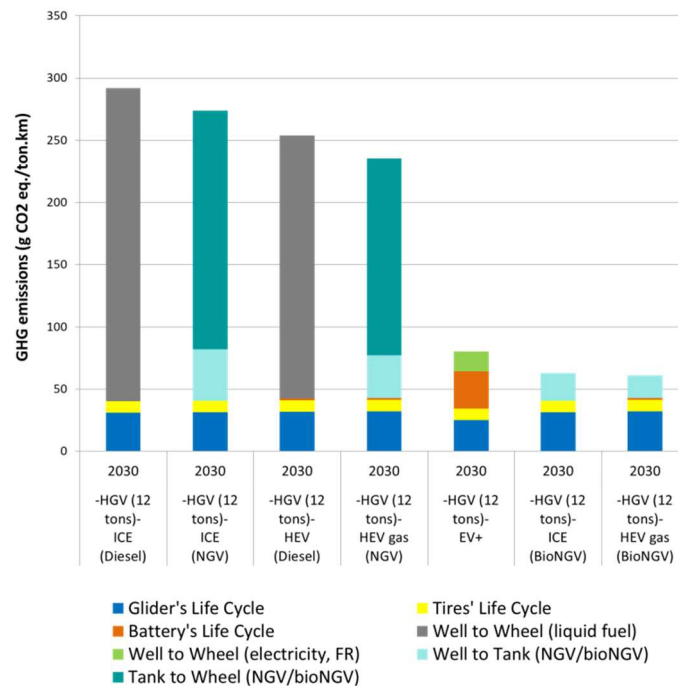
Figure 17: Potential impact on climate change for 12-ton heavy goods vehicles – 2030 time horizon
