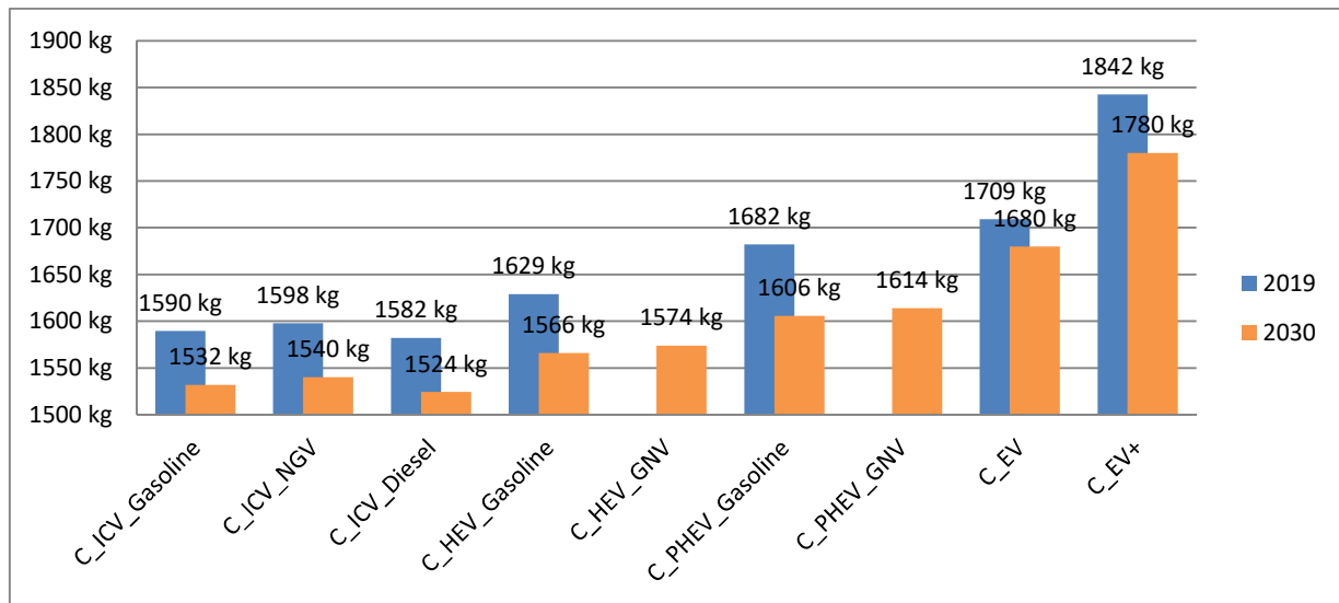
Figure 5: Change in simulated on-road weights [kg] between the 2019 and 2030 fleets of the C segment
