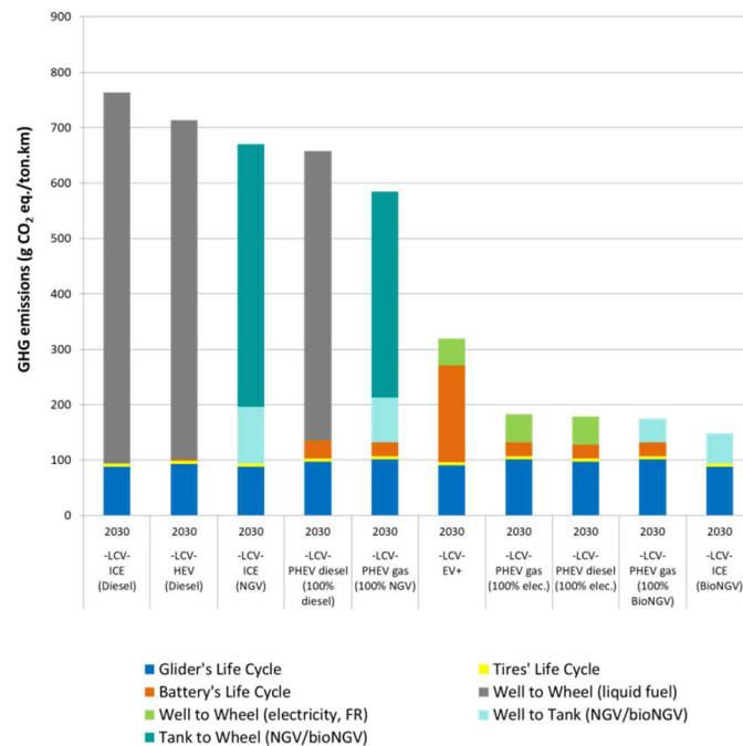
Figure 15: Potential impact on climate change for light commercial vehicles – 2030 time horizon
